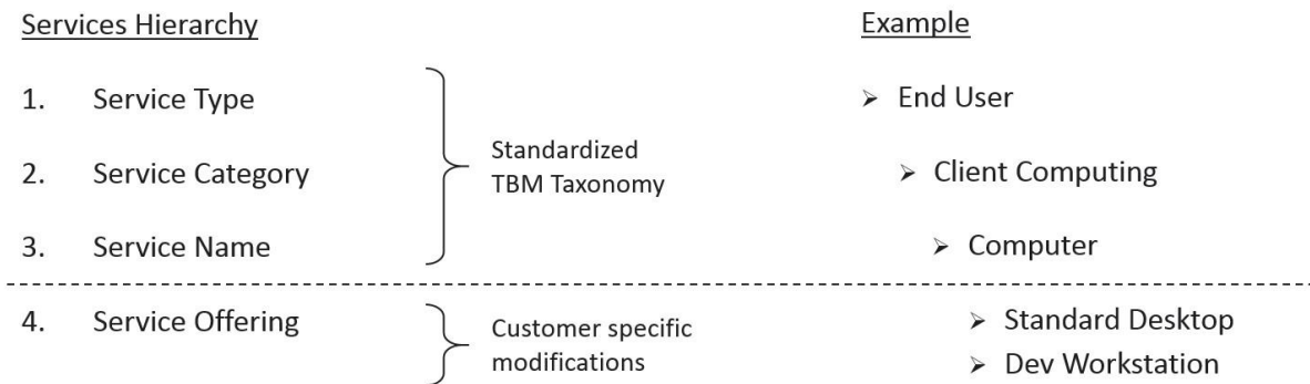
Figure 6: Services Hierarchy
